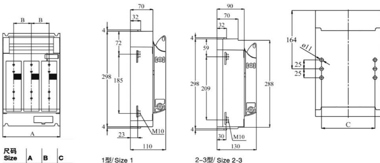
尺寸图/ Dimensions drawings 1-3型/ Size 1-3
