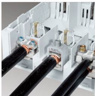
多种接线方式 A large range of connection possibilities
