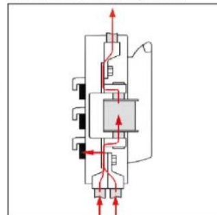
三极共分断， 方形设计， 安装于60mm母线系统的示意图 Drawing of the NH Fuse-Switch, 3-pole switching, horizontal design for busbar supply on a 60 mm busbar systems
